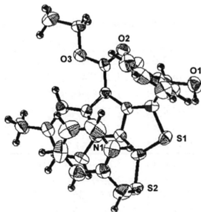
Figure 1. ORTEP drawing of 2j
